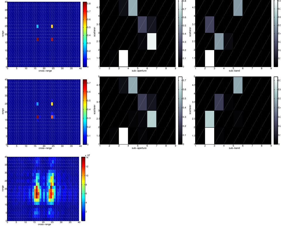
FIG. 5.5. Results with N_\omega = 8 frequency intervals, N_\alpha = 8 apertures and data contaminated with 20% noise. On the top row show the true reflectivity as a function of location (left) and direction (middle), and frequency (right). In the middle row we show the reconstructed reflectivity with the MMV algorithm. The plot in the bottom row is the migration image. The axes in the left images are cross-range and range in meters. The abscissa in the middle and right plots are the sub-aperture and sub-band index and the ordinate is the index of the scatterer (from 1 to 4).
