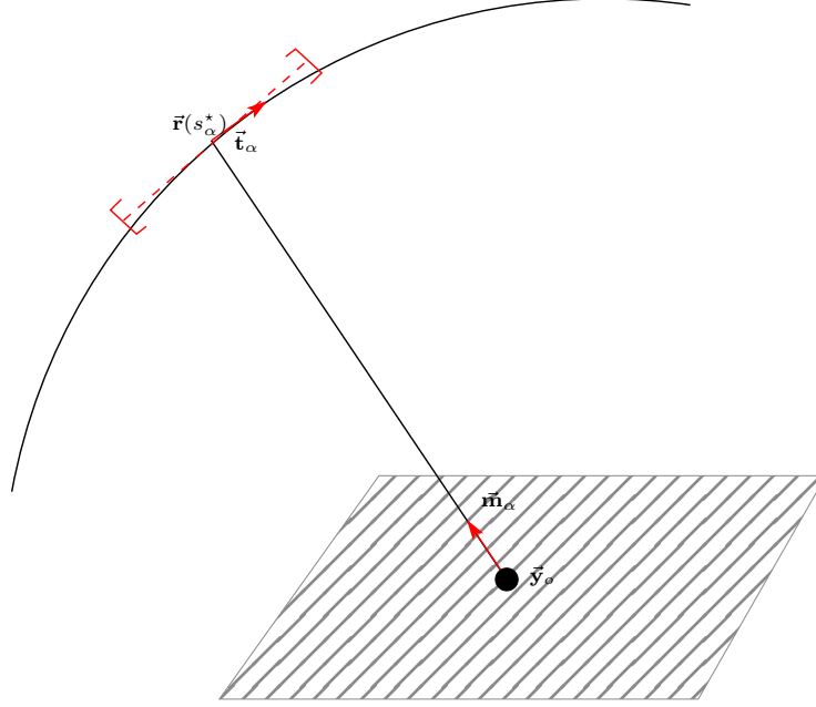
FIG. 3.1. Schematic of the geometry for one sub-aperture centered at the location \bar{\mathbf{r}}(s_q^*) of the receive-transmit platform.
