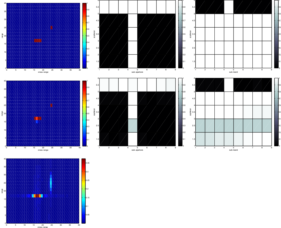
FIG. 5.7. Results with N_\omega = 8 frequency intervals, N_\alpha = 8 apertures and data contaminated with 20% noise. On the top we show the true reflectivity as a function of location (left), direction (middle), and frequency (right). The reflectivity is supported in 5 pixels, four of them are adjacent and represent an extended scatterer, which is frequency independent. The other pixel supports a small scatterer with frequency dependent reflectivity. In the middle row we show the reconstructed reflectivity with the MMV algorithm. The plot in the bottom row is the migration image. The axes in the left images are cross-range and range in meters. The abscissa in the middle and right plots are the sub-aperture and sub-band index and the ordinate is the index of the pixel in the support of the scatterer.
