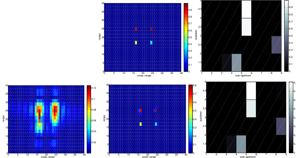
FIG. 5.4. Results for a single frequency sub-band and \mathcal{N}_\alpha = 8 consecutive, non-overlapping sub-apertures. On the top we show the true reflectivity as a function of location (middle) and direction (right). On the bottom we show the reconstructed reflectivity with 20% additive noise. Left plot is the migration image, middle plot is the MMV image and the right plot is the directional dependence of the reflectivity reconstructed with the MMV algorithm. The axes in the left images are cross-range and range in meters. The abscissa in the right plots are sub-aperture index \alpha = 1, \dots, \mathcal{N}_\alpha and the ordinate is the index of the scatterer (from 1 to 4).
