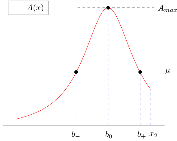
FIGURE 3. An example of a finite potential barrier accompanied by an infinite well on the left and a finite well on the right.
