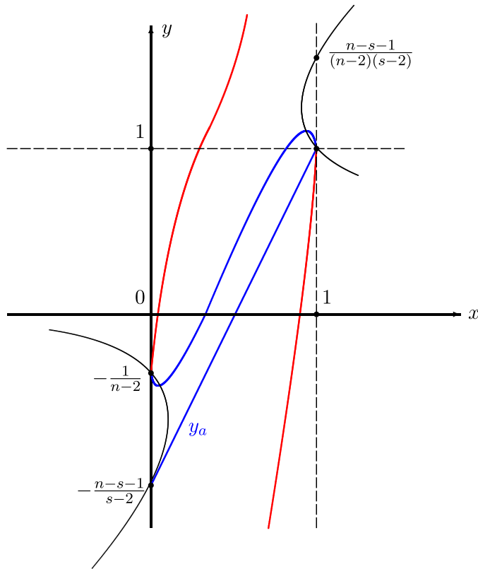
Fig. 3. Case n > 3 and 2 < s < \frac{3n-5}{n-1} . Connecting orbits are in blue and blowing up ones in red. (For interpretation of the references to colour in this figure legend, the reader is referred to the web version of this article.)
