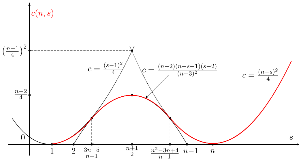
Fig. 1. Best constant (in red) for n > 3, s > 1 . (For interpretation of the references to colour in this figure legend, the reader is referred to the web version of this article.)
