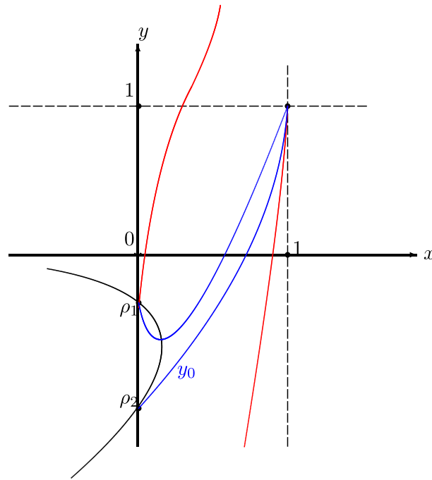
Fig. 2. Either n = 2, 3 and 1 < s < \frac{n+1}{2} or else n > 3 and 1 < s < \frac{3n-5}{n-1} . Connecting orbits are in blue. Blowing up ones in red. (For interpretation of the references to colour in this figure legend, the reader is referred to the web version of this article.)
