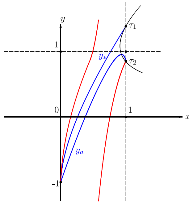
Fig. 4. Either n = 2, 3 and \frac{n+1}{2} < s < n or else n > 3 and \frac{n^2-3n+4}{n-1} < s < n . Connecting orbits are in blue and blowing up in red. (For interpretation of the references to colour in this figure legend, the reader is referred to the web version of this article.)
